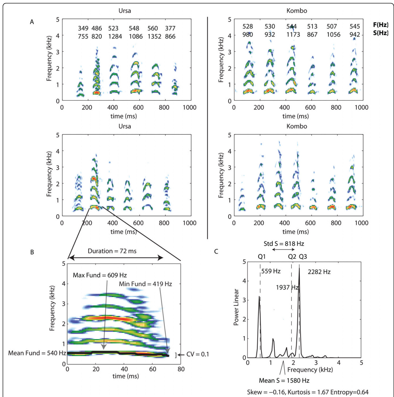
Figure 1 Acoustic structure of the hyena's giggle (laughing) call. A. Two giggle bouts emitted by two different individuals (Ursa and Kombo). The mean fundamental F(Hz) and the spectrum mean S(Hz) for each giggle note is shown on top of its spectrographic representation for the giggle bouts in the first row. Ursa is a subordinate animal while Kombo is a dominant animal. Ursa is a 10 yr old female and Kombo is a 9 yr old female. They are both control animals (no hormonal treatment). The sounds of the giggle bouts for Ursa are available as Additional Files 1 and 2. The sounds of the giggle bouts for Kombo are available as Additional Files 3 and 4. B. Spectrogram of the second giggle note from the bout for Ursa shown in the lower panel. The fundamental frequency is underlined in black. From this time varying fundamental frequency, we extracted the mean, the minimum and maximum values as well as the coefficient of variation (CV). The values for this note are shown on the plot. C. Frequency spectrum of the giggle note shown in B. From the frequency spectrum, we obtained the mean frequency, standard deviation, skew, kurtosis, entropy and the three frequency values that delineate the quartiles in energy. The values for this note are shown on the plot (see main text for additional details about fundamental calculation and measurements of acoustic parameters)
